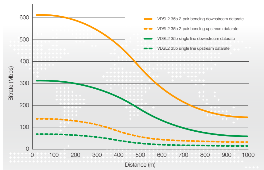
Figure 1: VDSL2 profile 35b single line and bonding performances.
